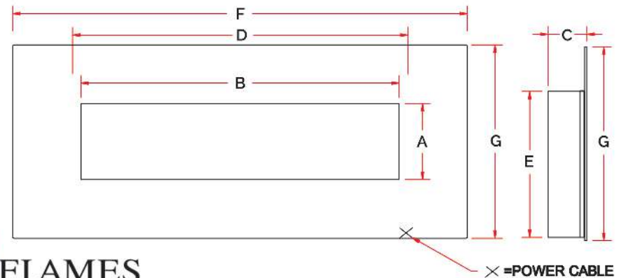
AL60CLX2 TECHNICAL DRAWING SHOWN
